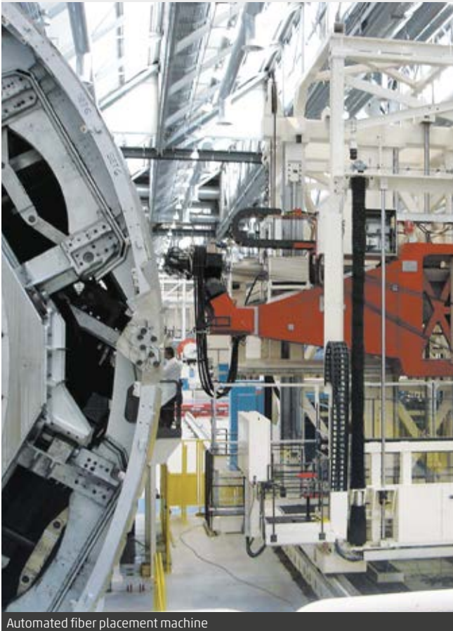
Automated fiber placement machine
