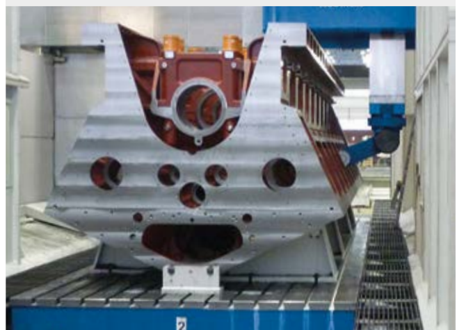
Vertical milling machine with travelling table for diesel engines
